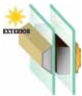
SDL Pyramid Bar with Wood Interior and Internal Shadow Bar
