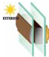
7/8" SDL Contoured with Wood Interior and Internal Shadow Bar
